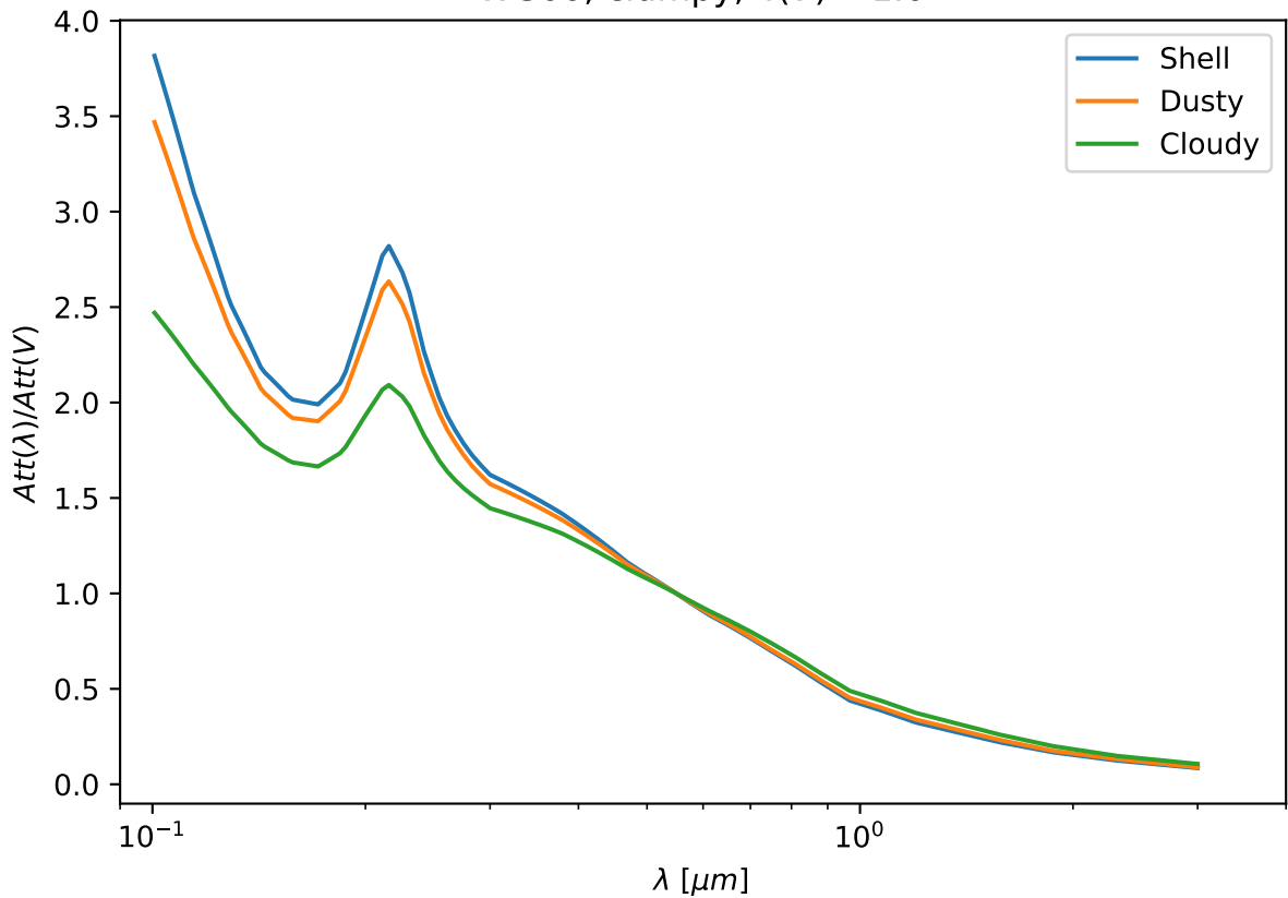
WG00, clumpy, \tau(V) = 1.0
