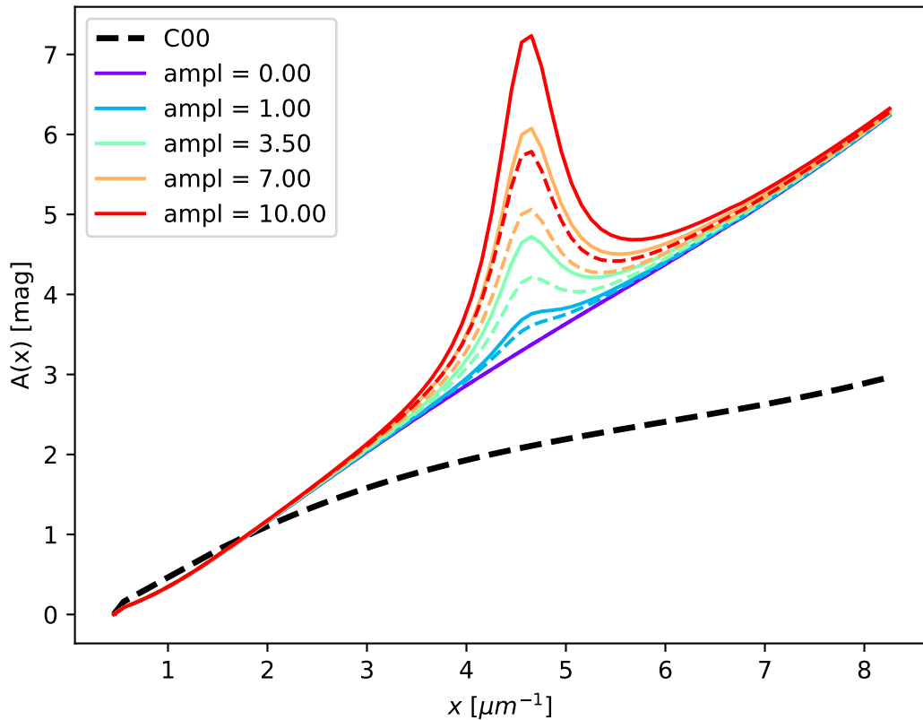
N09 and SBL18 with varying UV bump amplitudes
