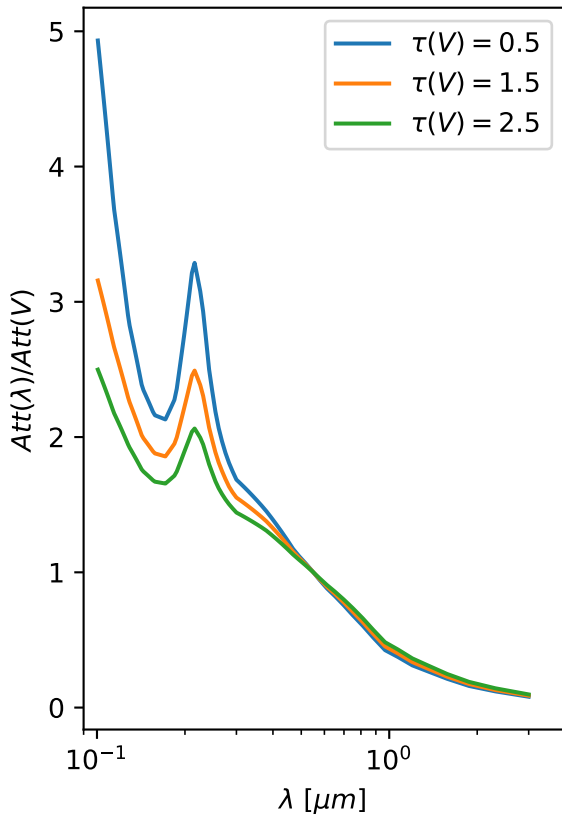
Normalized Attenuation
