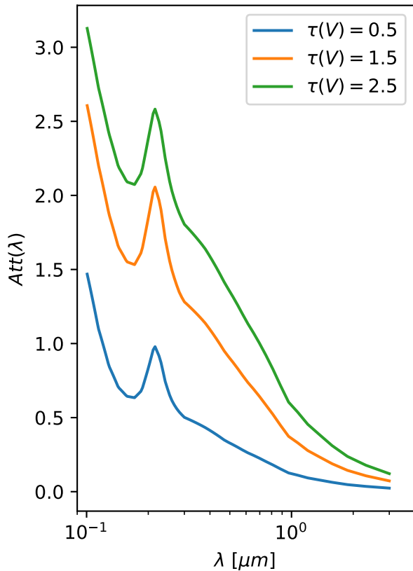
Total Attenuation
