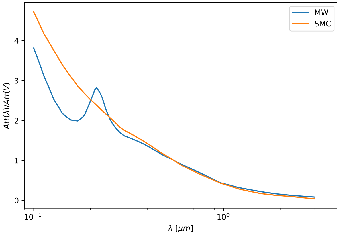
WG00 Shell, clumpy, \tau(V) = 1.0
